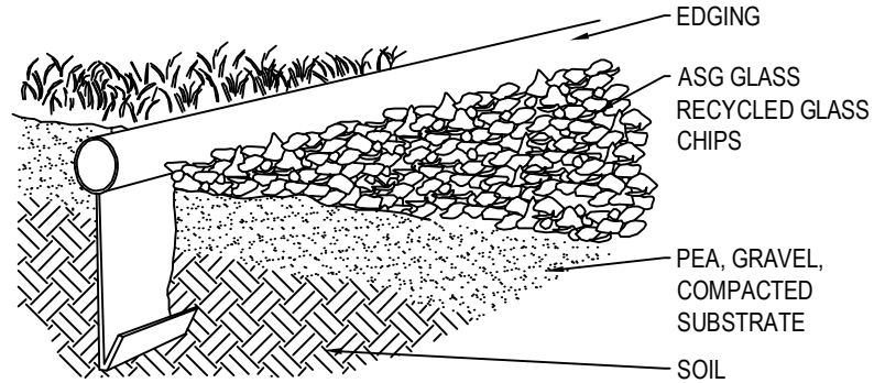
EDGING APPLICATION - ISOMETRIC
