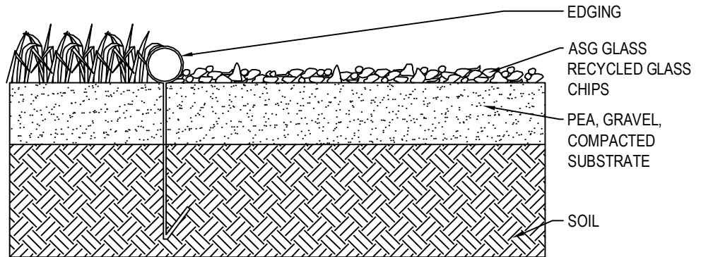
EDGING APPLICATION - SECTION
