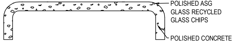
CONCRETE BENCH APPLICATION - SIDE VIEW
